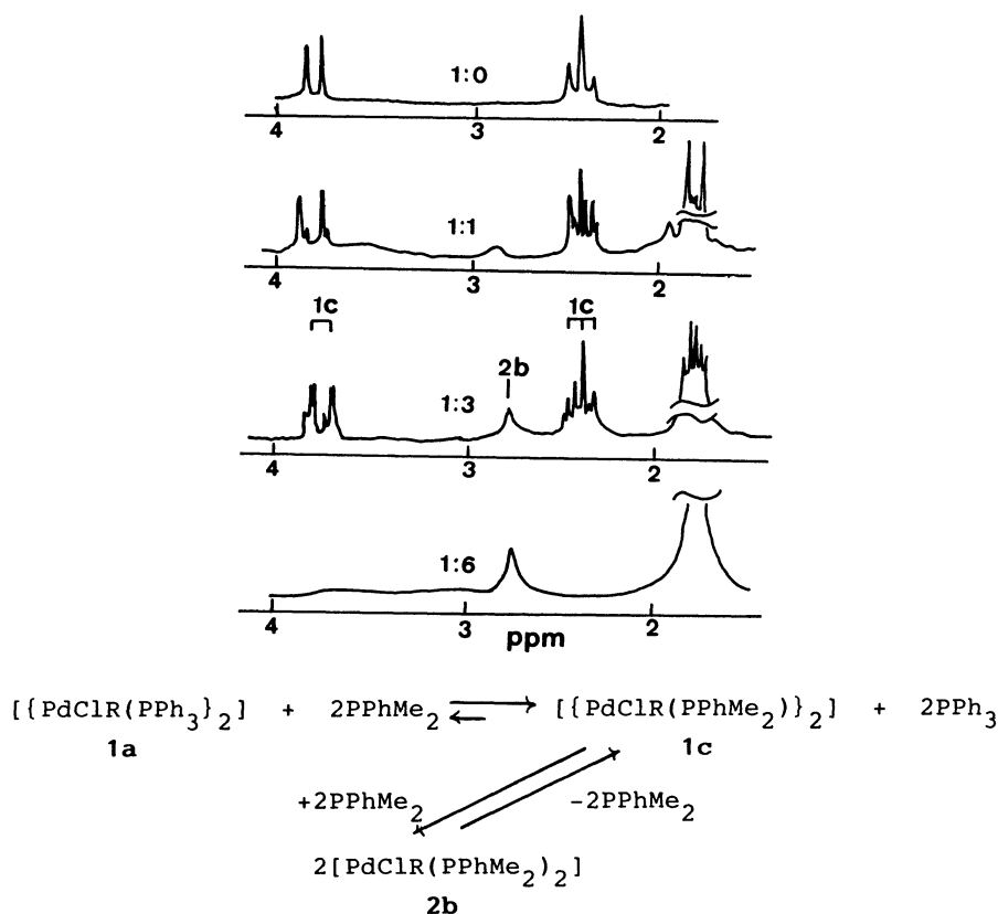
Fig. 4. The methylene-proton signals from [\{\text{PdCl}(\text{C}_5\text{H}_4\text{N-2-CH}_2)\text{PPh}_3\}_2] ( 1a ) in \text{CD}_2\text{Cl}_2 at room temperature in the absence and in the presence of one equivalent, three times, and six times molar amount of phenyldimethylphosphine. In the reaction scheme R represents the 2-picolyl ligand.
